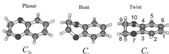
Figure 1. Structures of the three lowest energy structures of BZD: planar ( C_{2v} ), boat ( C_s ), and twisted ( C_2 ), along with the atomic numbering.
