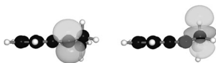
Figure 4. Side view of the p -type oxygen lone pair (left) and the antibonding \sigma^* orbital of the adjacent CH 2 group (right) in ground-state BZD.
